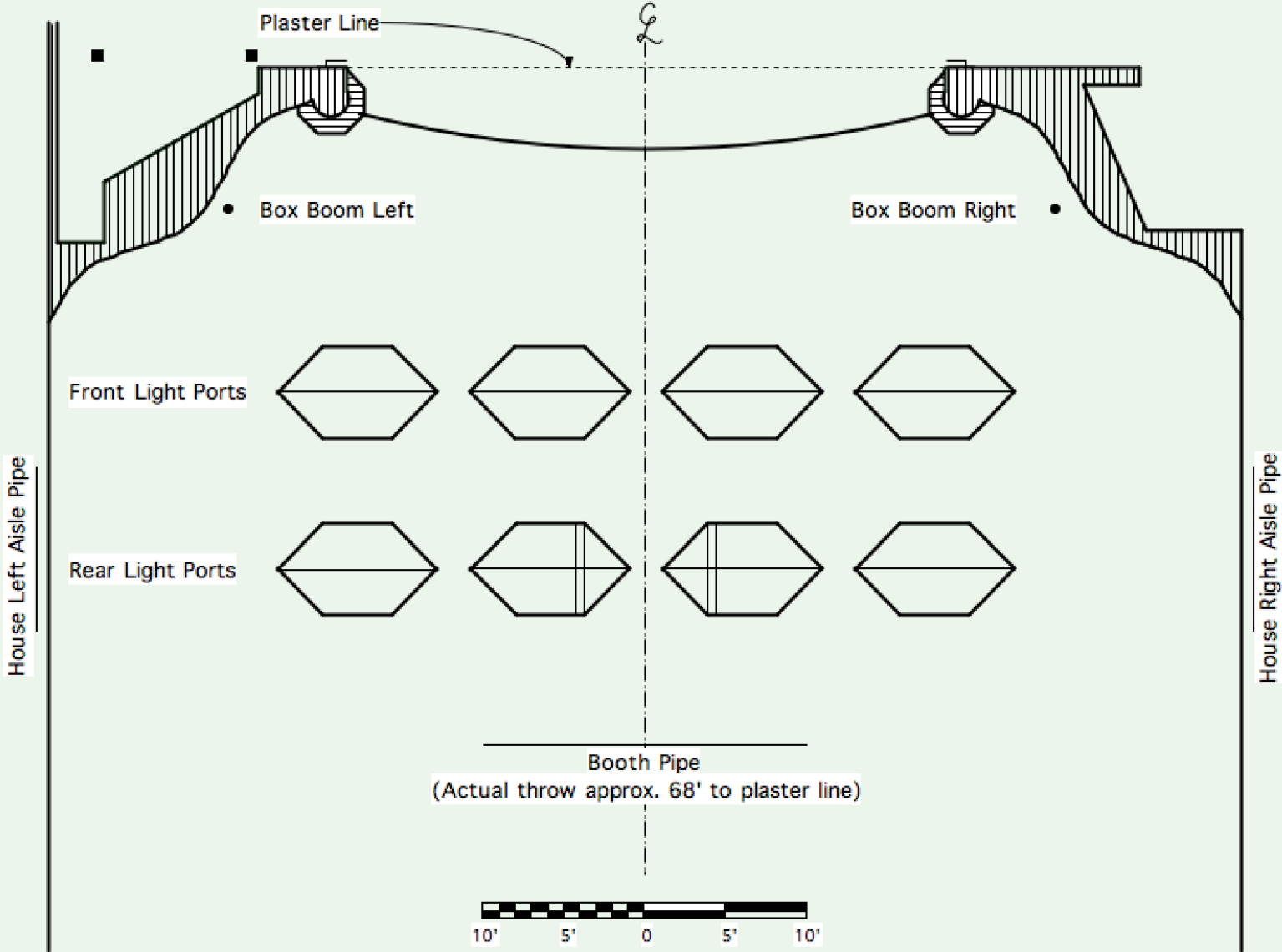
LOBERO THEATRE AUDITORIUM CEILING PLAN
